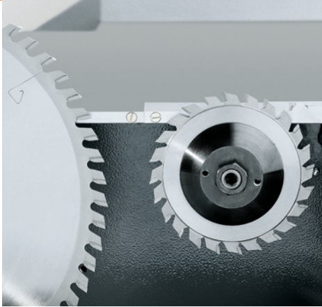
The scorer. Separate 0.37 kW scoring motor with on/off switch.
