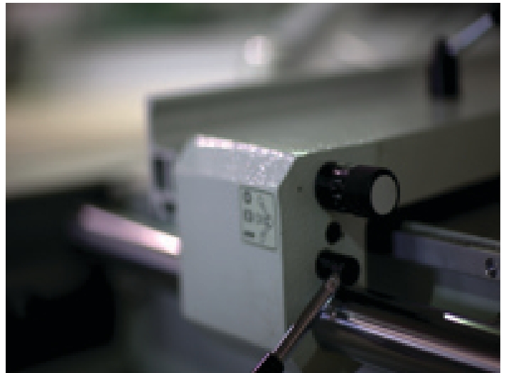
Rip Fence with Micro Adjustment Feature
