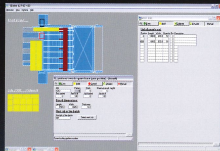
Simulazione grafica e in tempo reale delle fasi operative (RTG System). Graphic simulation in real time of the various operating phases (RTG System).
