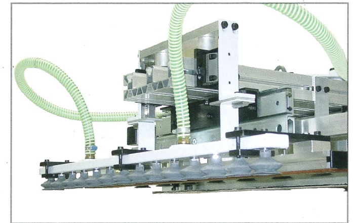
Detail des Saugrahmens des Portalroboters Detail of suction frame of gantry robot
