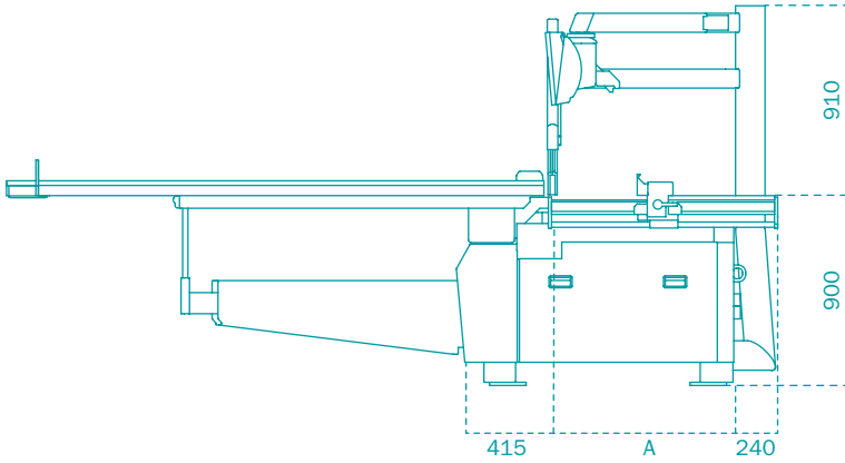
T70 | Side view
