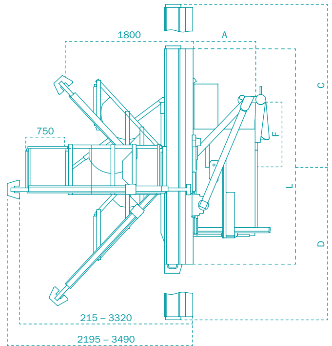
T70 | Plan view
