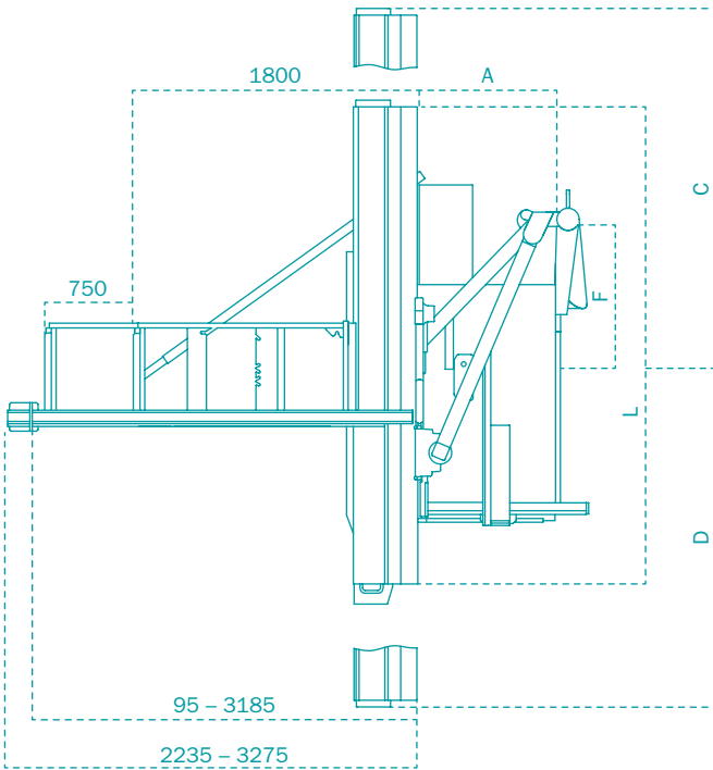
T70 | Plan view
