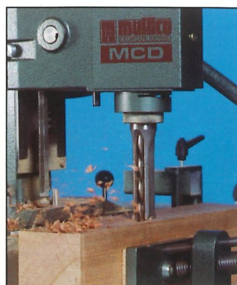
Multico's hollow chisel system gives deep, precise mortises in both hard and soft wood, MDF and other materials.
