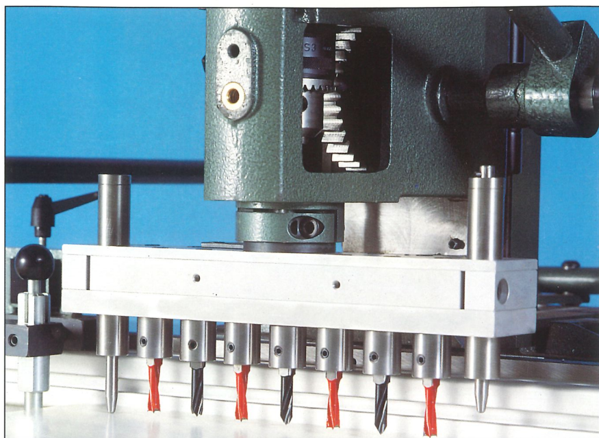
Multico 7 spindle multi-boring head using the 32mm system can be fitted in minutes. The head incorporates spring loaded stops at each end for locating from existing holes or the edge of panels.
