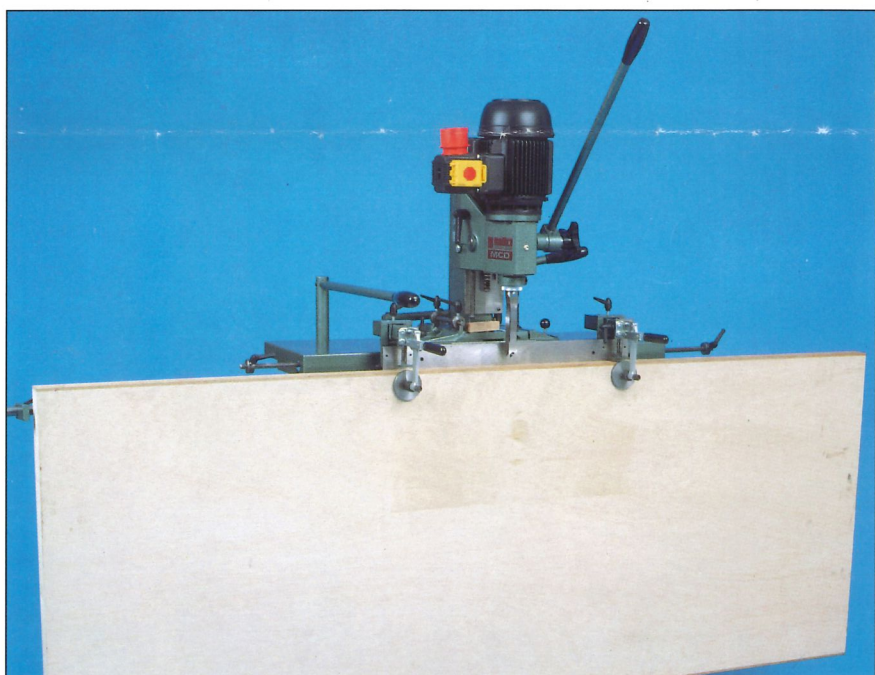
MCD in door mortising mode accepting all standard door sizes.
