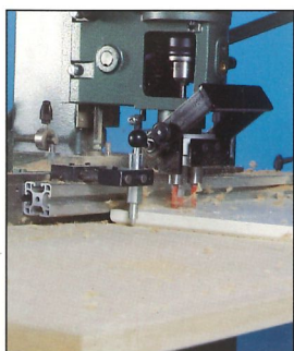
The stops system shown comprises a fence rail, two stops with spring loaded action for holes or edges and an extension table.
