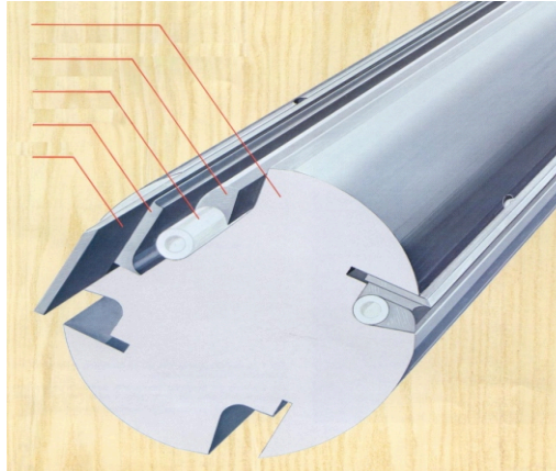
cuttershaft with hydrostatic clamping of knives
