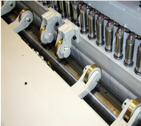
Knife adjusting device
