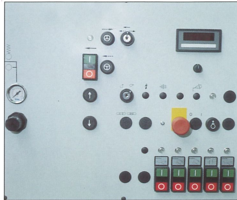
Control panel with optional LED display for inverter feed drive unit 6-36m/min.
