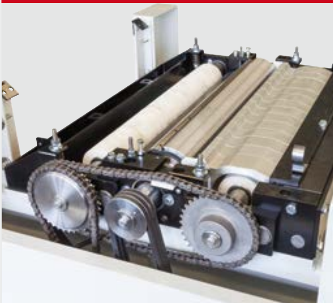
Roller mill
