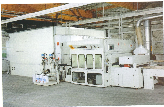
Spray plant with vertical dryer
