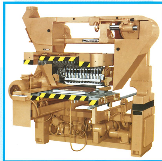
Stuhlsitzschleifmaschine Shaped surface sanding machine
