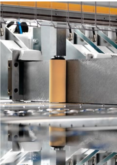
Feeding table with pneumatic pressure roller for exact angular cuts even of long components.
