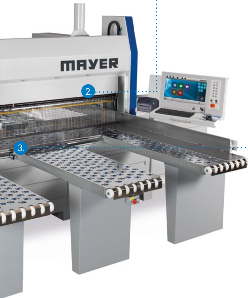
Pneumatically controlled vertical fastening unit for strip cuts.
