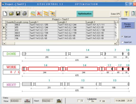
BL100A: Software zur Maschinensteuerung BL 100A: Software for machine control
