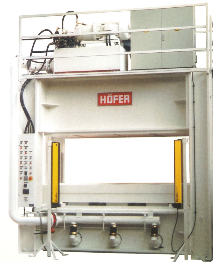
Formpresse 500 to
