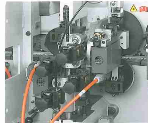
Tiltable fine trim unit with pneumatic adjustment.
