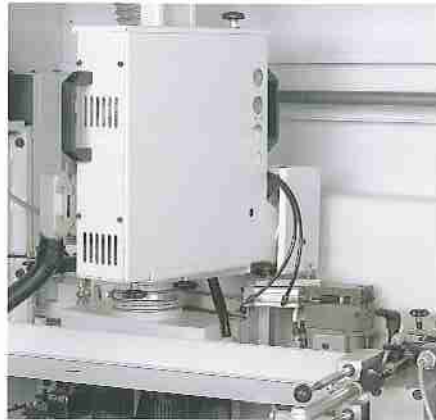
High availability and optimum glue quality due to the Quickmelt gluing station.
