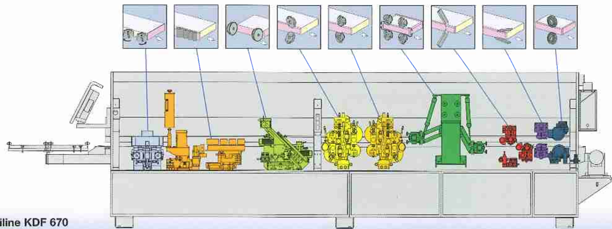
Profiline KDF 670
