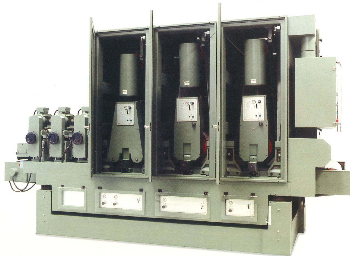
Wide calibrating machine P.C. controlled model 90 CCT/1900
