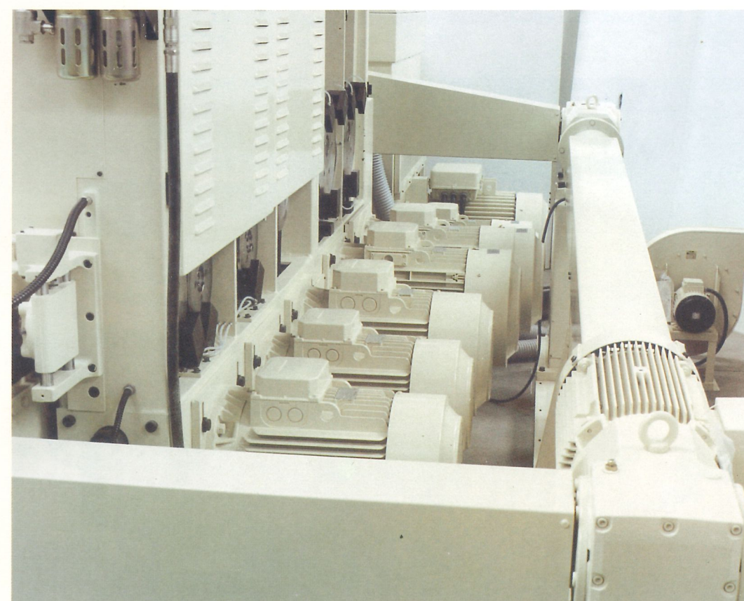
Total machine power HP. 440. Feed speed 90 m/minute. Drive motor HP. 40.
