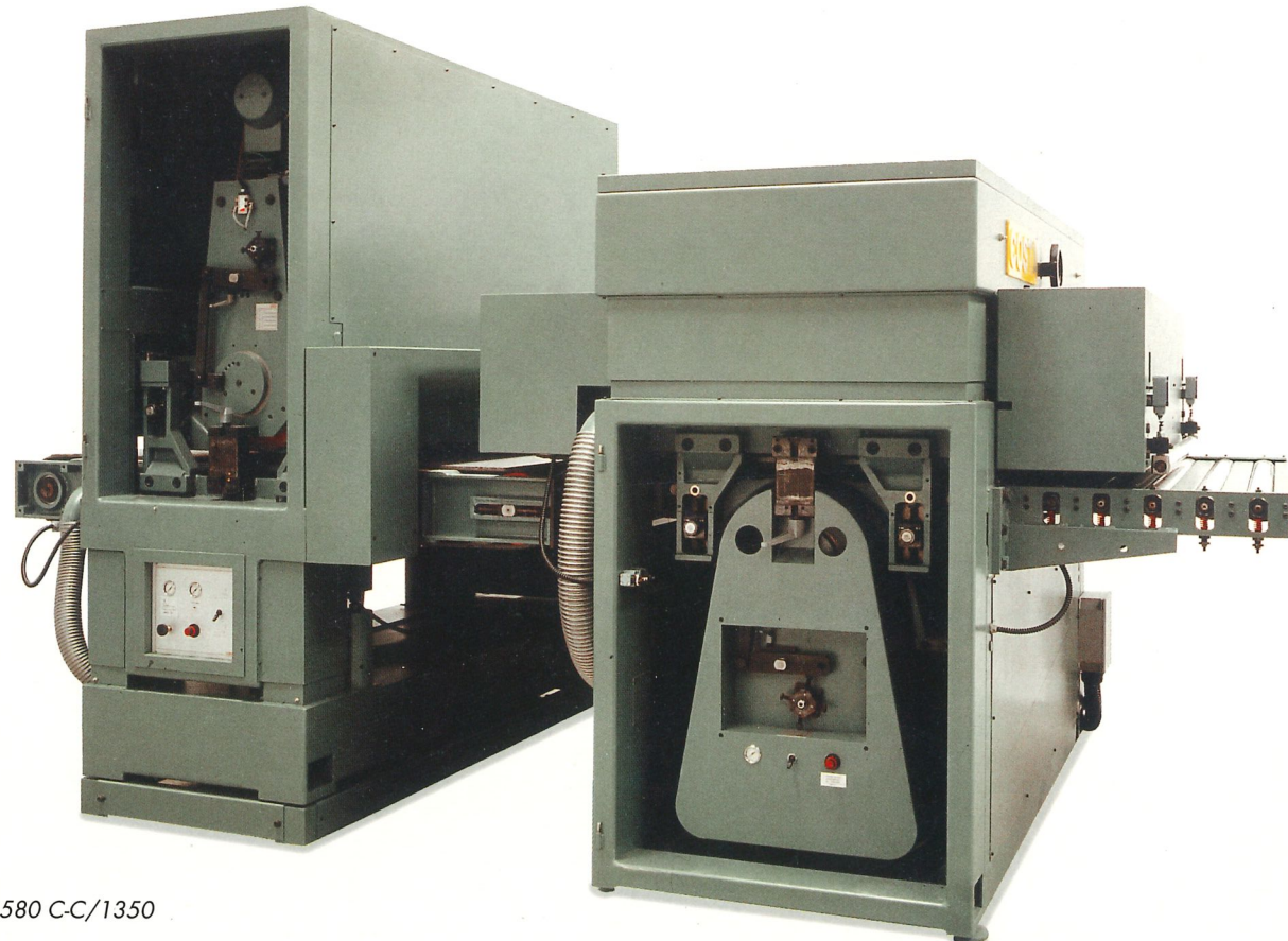
Opposed heads model PRISMA C-C/1350
